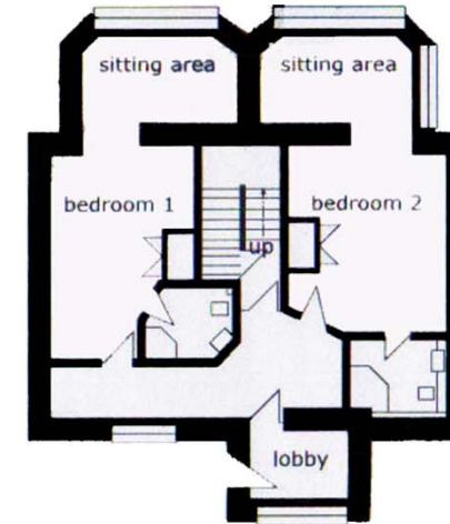
Floorplans
